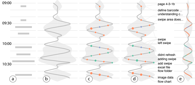
Figure 5. The process of generating ThreadPulse. (a) An adaptive binning approach divides the time frame into multiple N -minute time slots (gray bars indicate message intensity values). (b) A volume chart and a zig-zag curve is drawn to present message intensity across time. (c) Messages are depicted as circles along the curve. (d) Keywords of threads are placed on the side. (e) The coarse-level design of ThreadPulse hides details such as keywords and the number of messages in each time slot.
