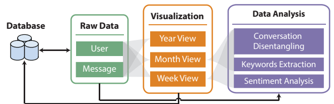
Figure 2. Overview of T-Cal architecture.
