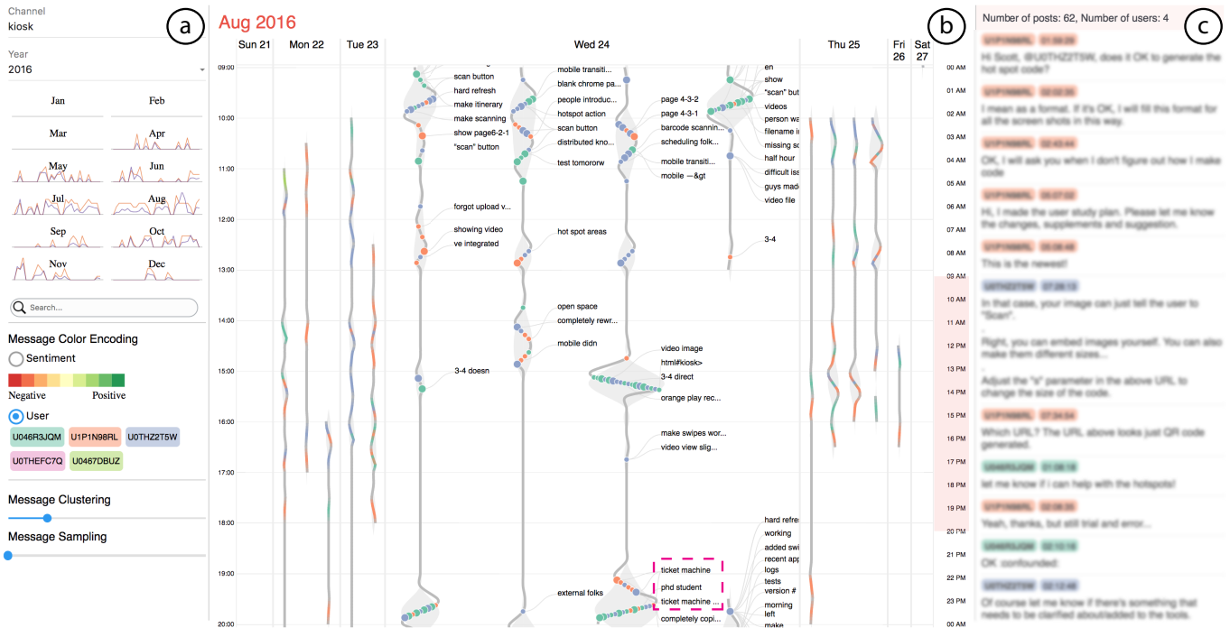
Figure 1. Using T-Cal to explore conversation data generated by team messaging platforms (e.g., Slack). (a) A Control Panel provides configurations for the entire system and entrances to view different datasets with different years and months. (b) A Content panel illustrates team conversational patterns at different time scales, including year, month, and week views. Here, the week of August 21, 2016 is shown with conversational threads presented by a novel visual design called ThreadPulse. (c) A Detail Panel allows users to browse raw messages of selected objects.
