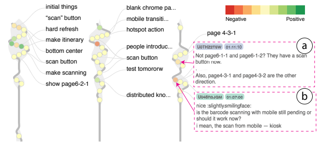
Figure 9. ThreadPulse with the color representing message sentiment. (a)(b) The raw data of two messages in red boxes, respectively.
