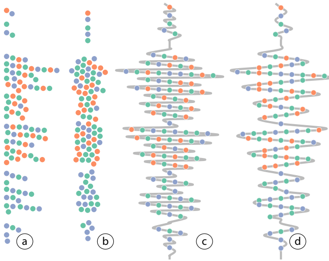
Figure 6. Design alternatives for ThreadPulse showing the same thread during the same time period. (a) A bee swarm chart. (b) The FluxFlow plot. (c) An initial curve-based design. (d) The final curve-based design used in ThreadPulse.
